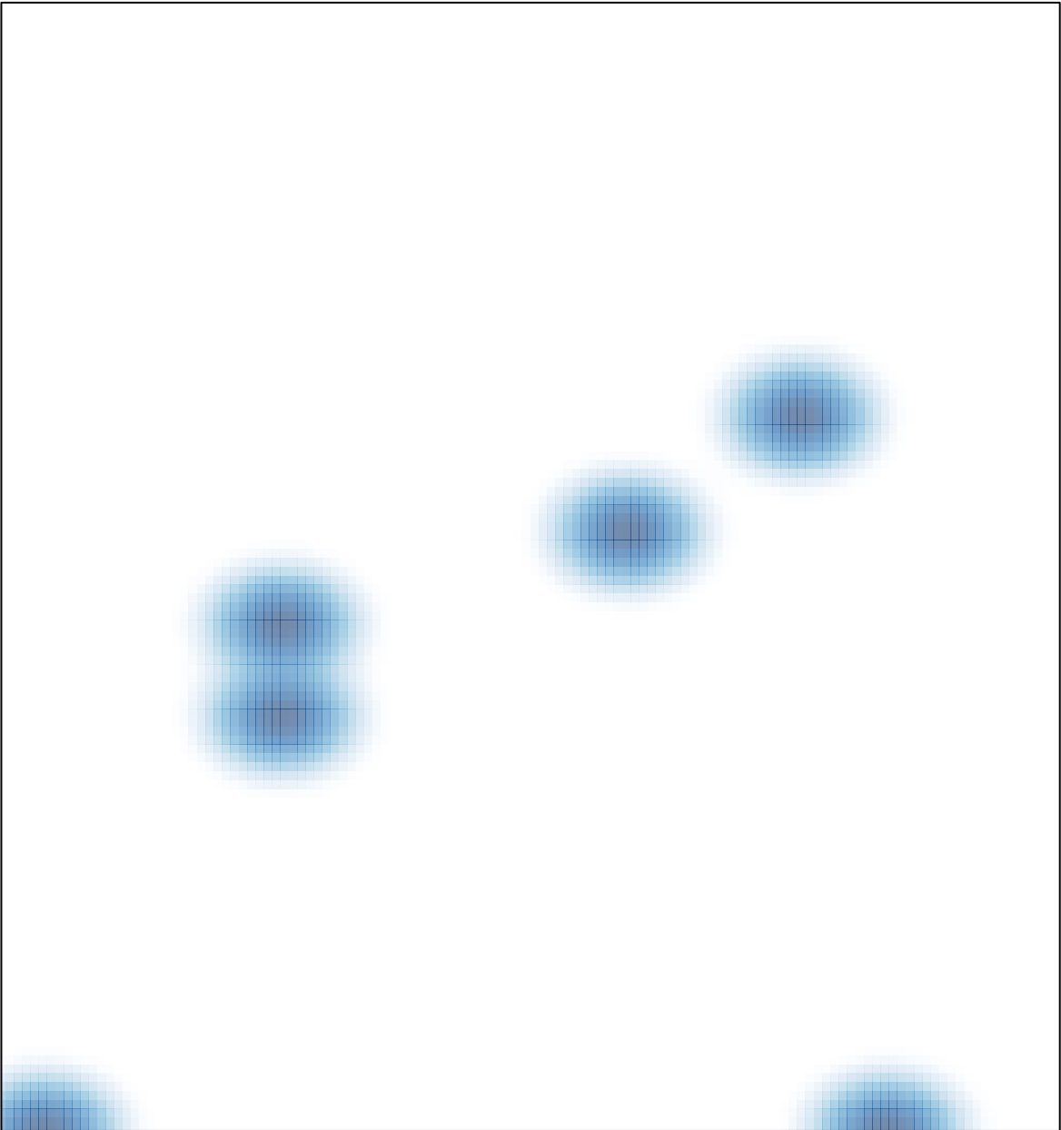
# features = 7 , max = 1
